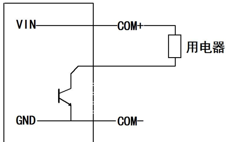
DAM0808-YD模块
